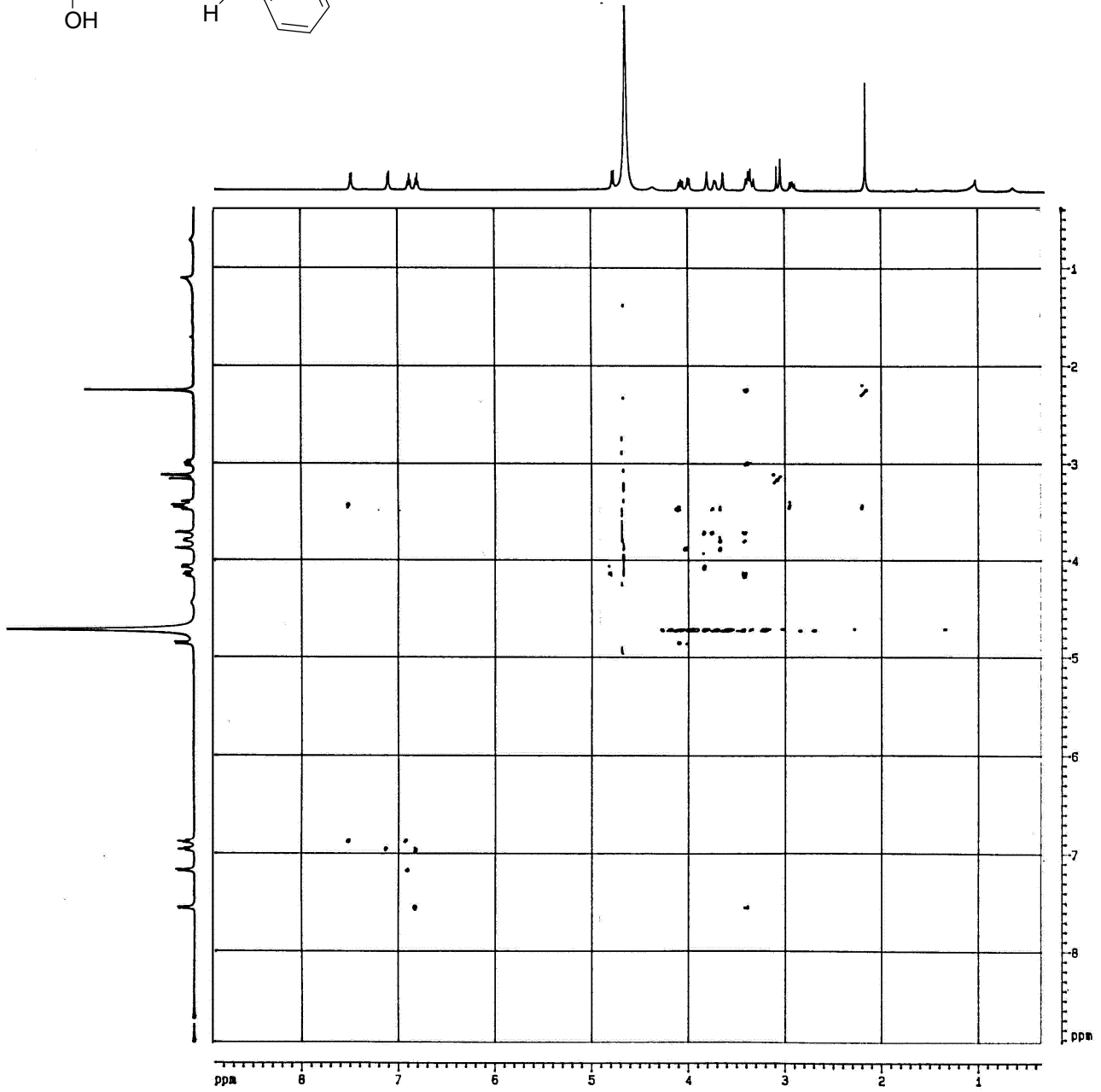
NOESY of compound 2
